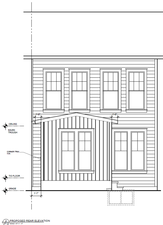
PROPOSED REAR ELEVATION SCALE: 1/4" = 1'-0"
